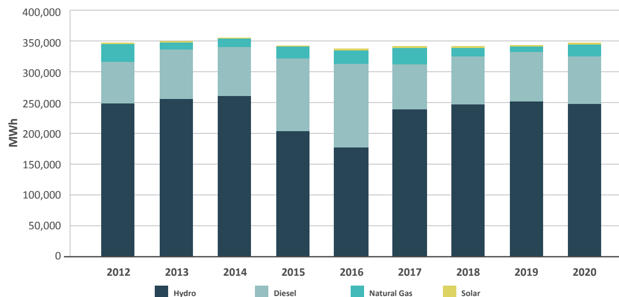
Figure 3. Utility power generation by source between 2012 and 2020
