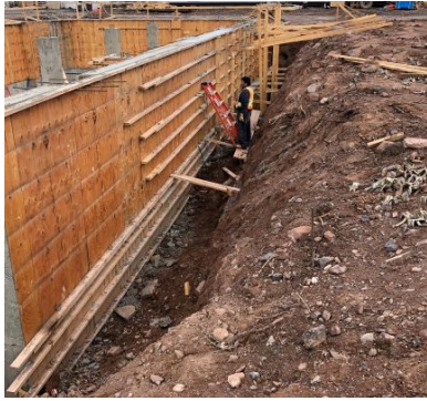
The foundation for a new diesel generating plant being installed in Łutselk'e. The new plant will have high efficiency generators and is located outside of the centre of the community, moving fuel storage away from Great Slave Lake as well as reducing noise and GHG emissions.
