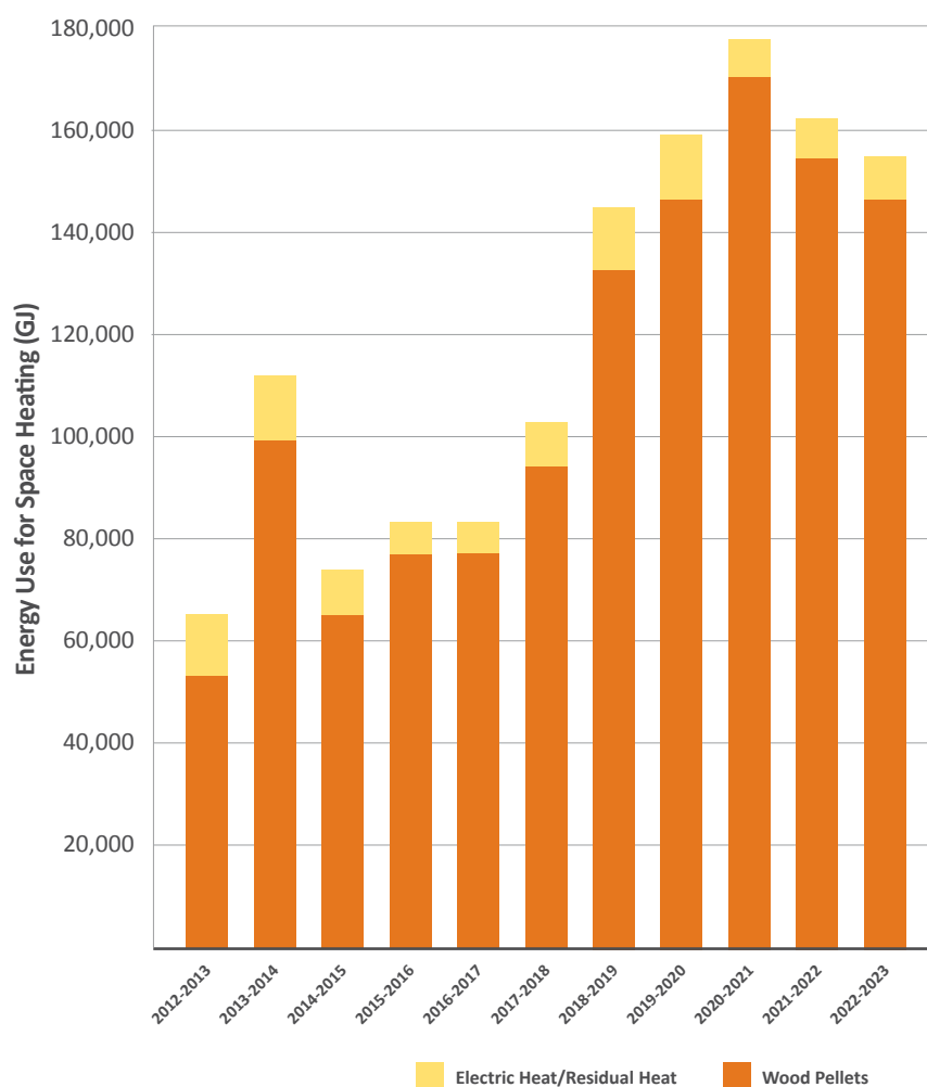
Figure 16. GNWT Space Heating Provided by Renewable Energy
